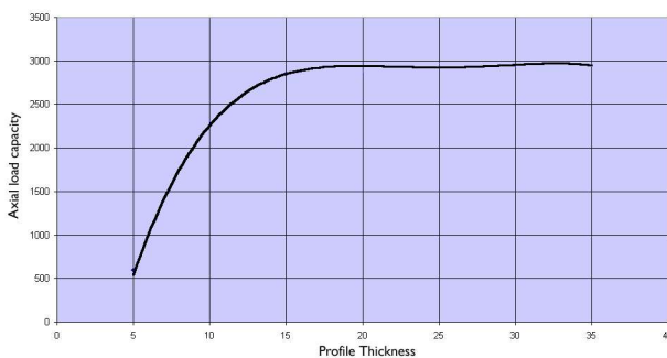
AXIAL LOAD CAPACITY ACCORDING TO PROFILE THICKNESS
