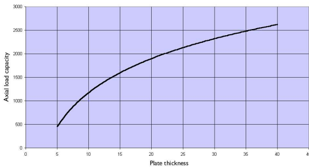
AXIAL LOAD CAPACITY ACCORDING TO PLATE THICKNESS
