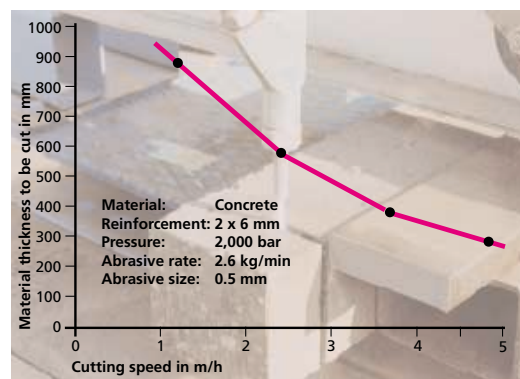
Approximated cutting speeds for structural steel and reinforced concrete
