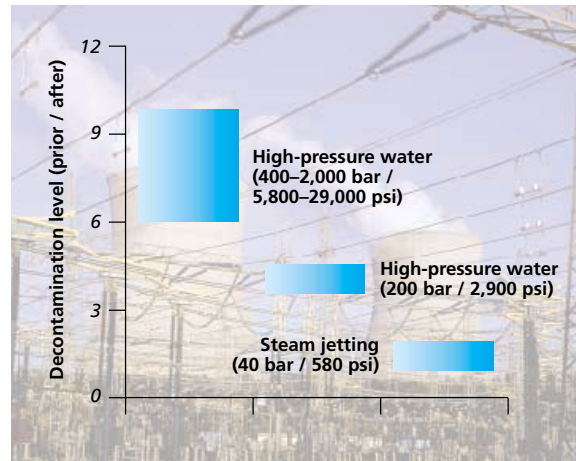
Decontamination of uranium rods (graphite)
