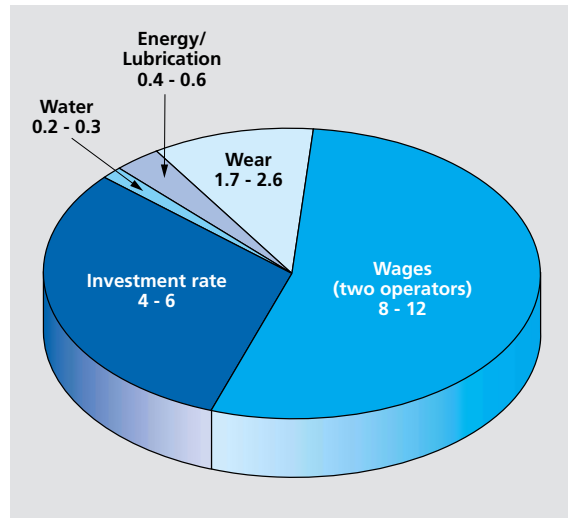
Cost structure for the decontamination of fire-damaged concrete including waste recovery (DM/m²; status 1998)
